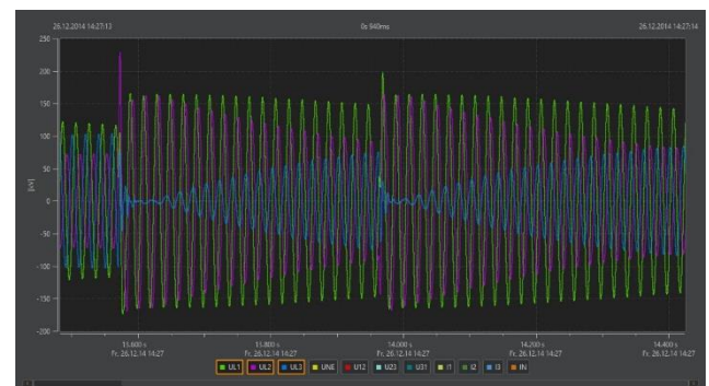
Figure 3 Oscilloscope image U1N, U2N, U3N
