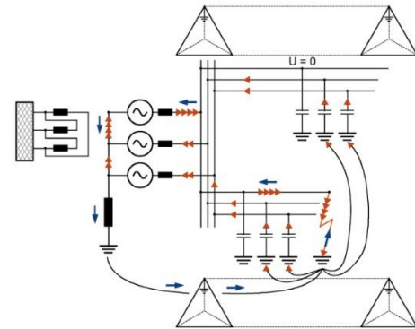
Figure 2 Compensated Network
