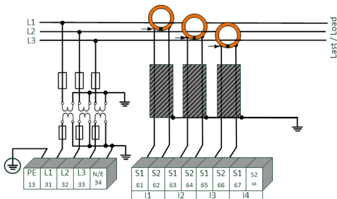
Example of PQI-DA smart connection with Rogowski coils in a 3-wire network
