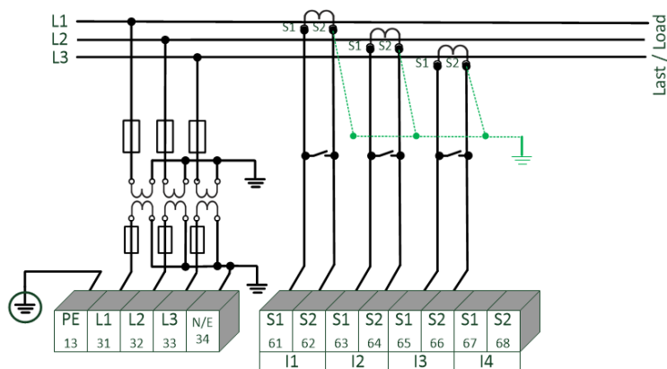
PQI-DE in 3-wire connection for medium and high-voltage via transformer
