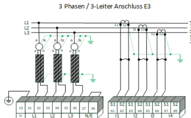
PQI-DE in 3-wire connection for medium and high-voltage via voltage sensors
