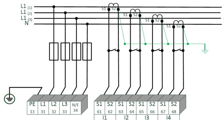
PFI-DE in 4-wire connection / 1-phase
