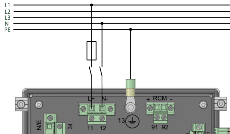
Example of connection to 230V AC with feature H1
