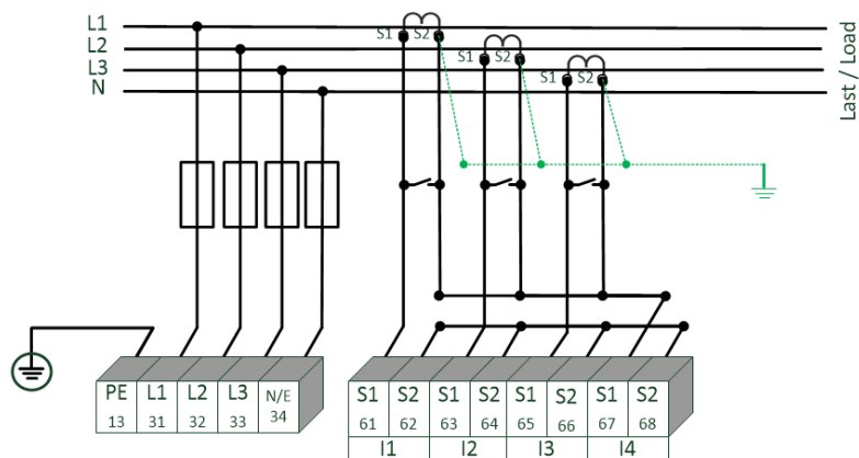
PFI-DE without neutral conductor Current transformer in 4-wire connection
