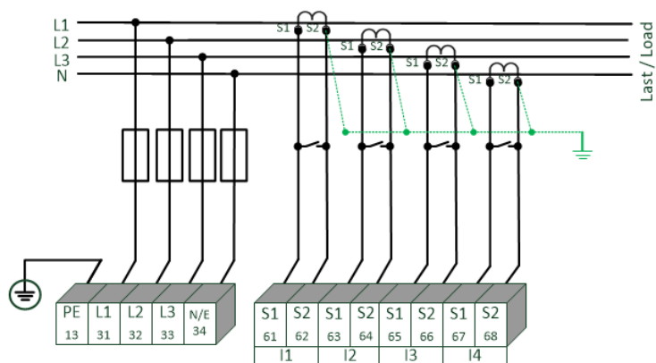
Example of a connection for a PQI-DE in a three-phase four-wire system
