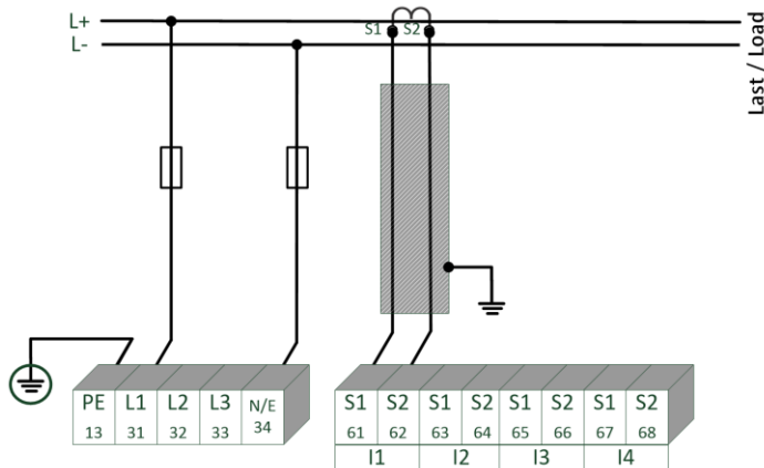
Example connection PQI-DE with current transformer with small signal output (e.g. 4 V)
