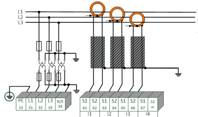
Example of PQI-DE connection with Rogowski coils in a 3-wire network
