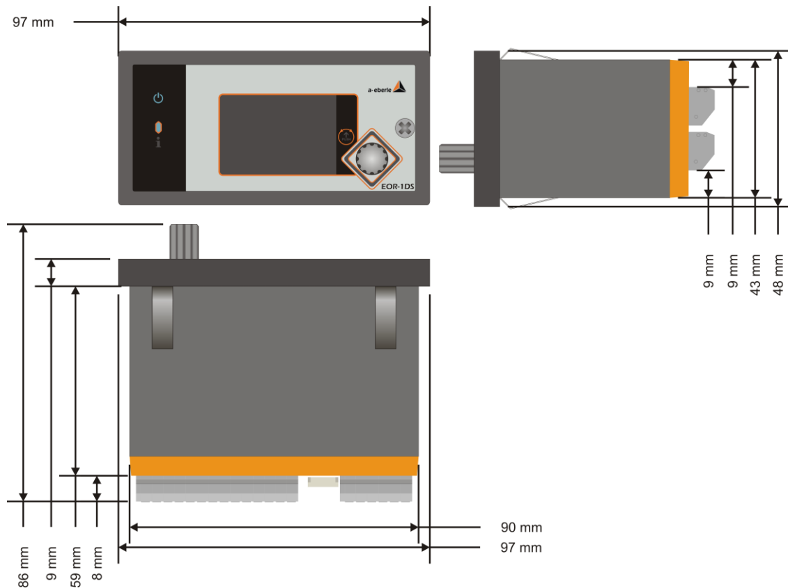
Figure 8: Dimensions EOR-1DS
